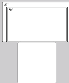
W7 L for 70"- 80" displays with up to 80 kg weight
